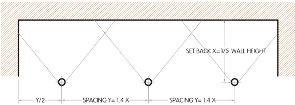
Wallwasher Optimal Spacing
