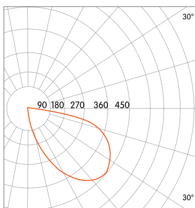
Steplight Asymmetric Distribution
